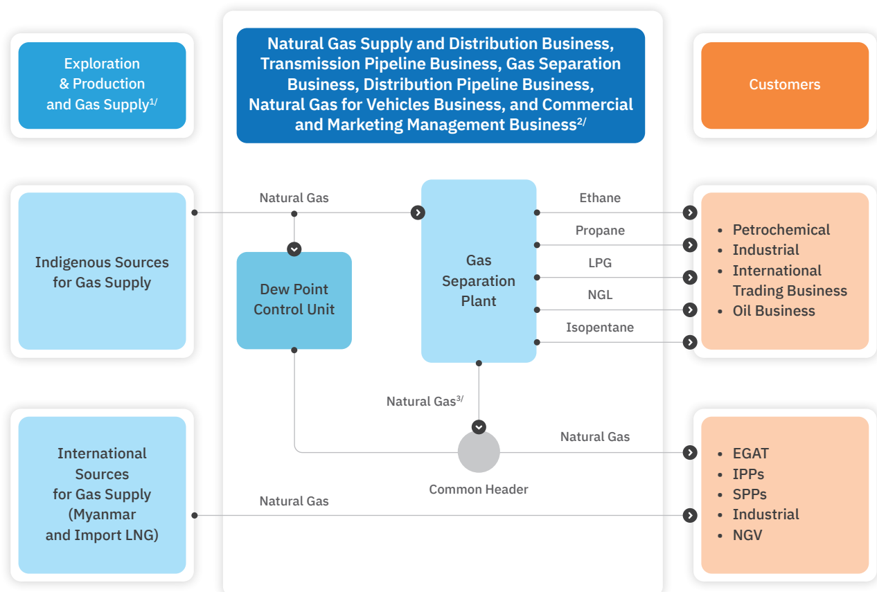
Diagram of PTT Group's Upstream & Gas Business Group
